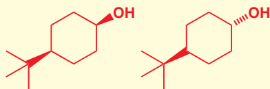
these diastereoisomers are achiral
