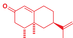
nootkatone supposed flavour principle of grapefruit
