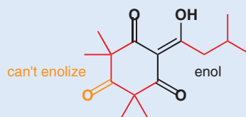
Leptospermeone (Callisto ® ) herbicide produced by the bottle-brush plant
