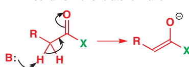
mechanism of enolate formation
