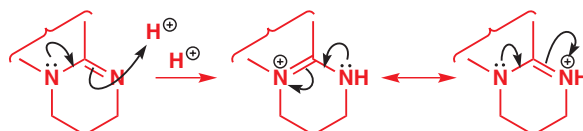
protonation of the amidine system
