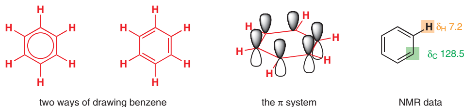
two ways of drawing benzene
