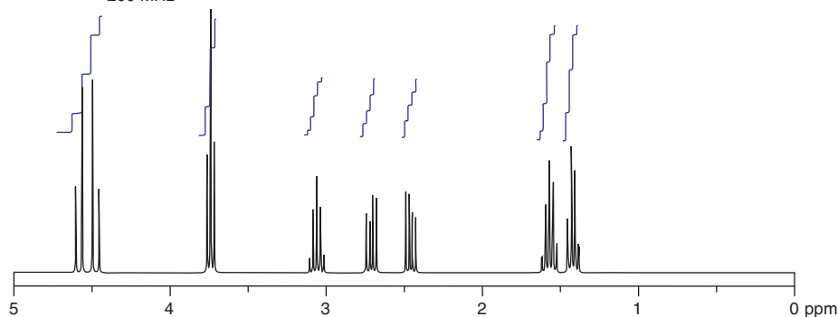
^1\text{H} NMR spectrum of product 200 MHz
