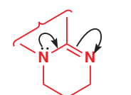
delocalization in the amidine system
