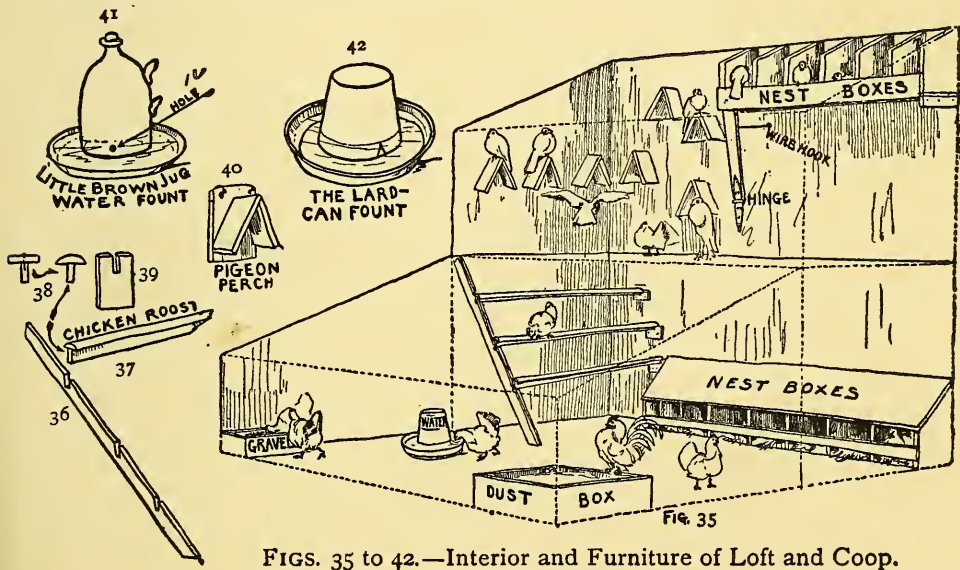
FIGS. 35 TO 42.—Interior and Furniture of Loft and Coop.
