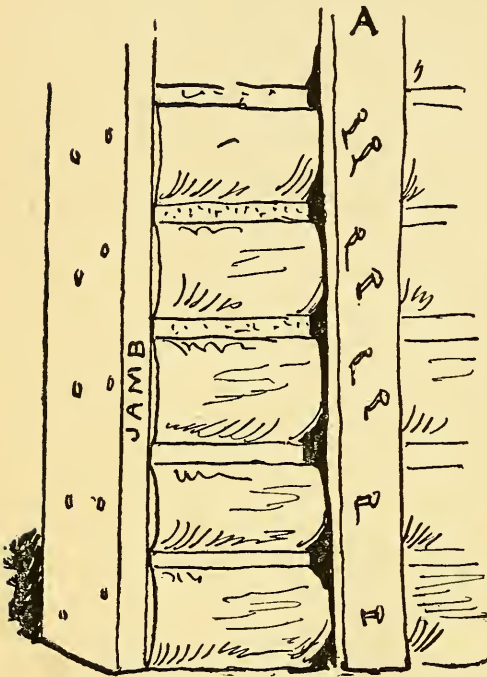
FIG. 99.—Binder and Jamb for Opening.
