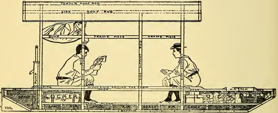
FIG. 117.—Cross-Section of Boat.
