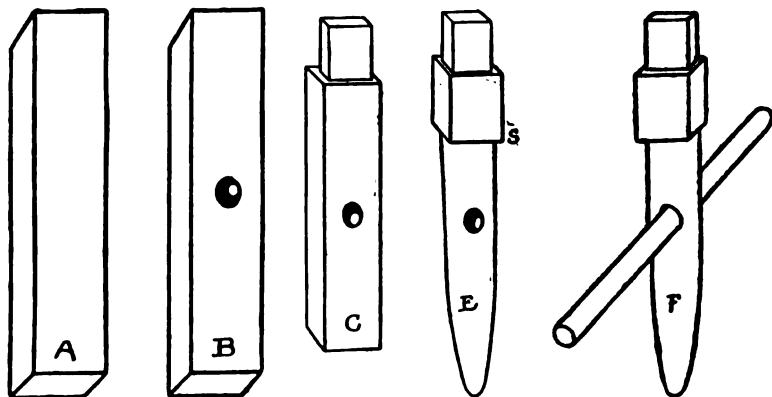
FIGS. 194, 195.—Stick for Rudder-post of Catamaran.
