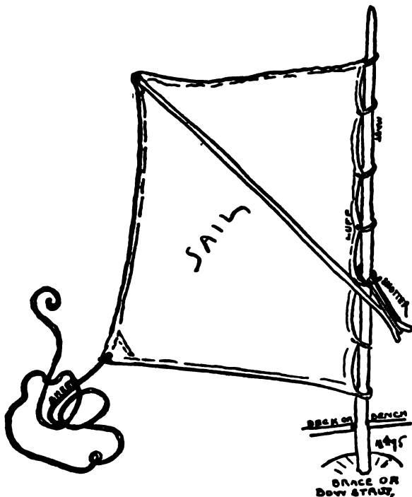
FIG. 18a.—Sail for Man-Friday.
