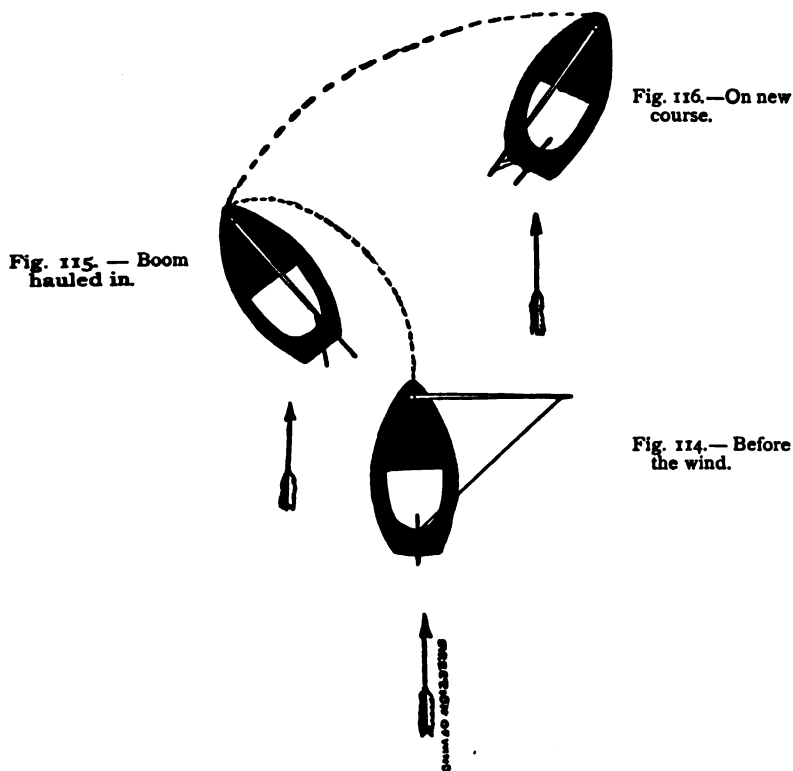
FIGS. 114, 115 and 116.—Jibing.
