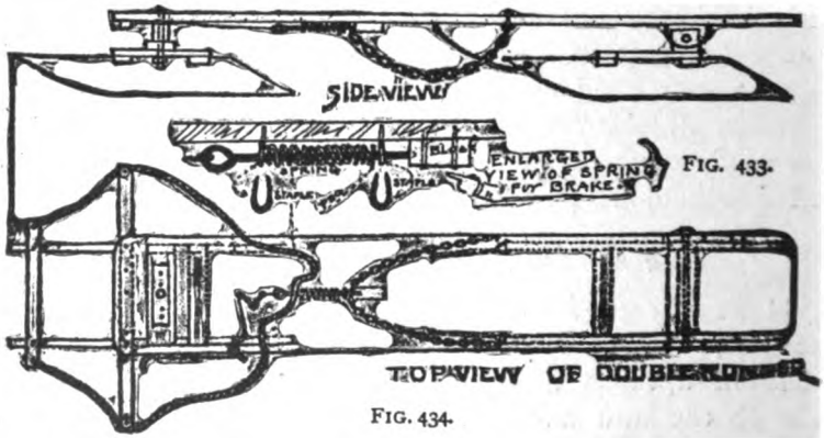
Working Plans for the Construction of Safety Double-Runner.
