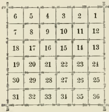
FIG. 191.—A common method of marking section corners. Used chiefly in the West.
