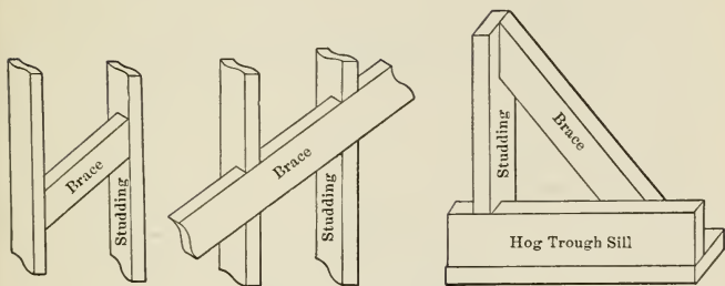
FIG. 78.—Studding braces.
