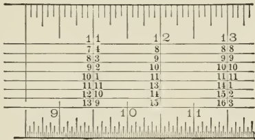
FIG. 114.—Board Scale.
