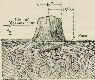
FIG. 69.—Charge placed too near surface.
