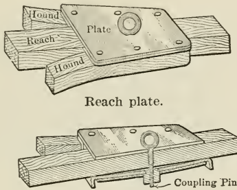
FIG. 142.—Sectional view of reach plate.
