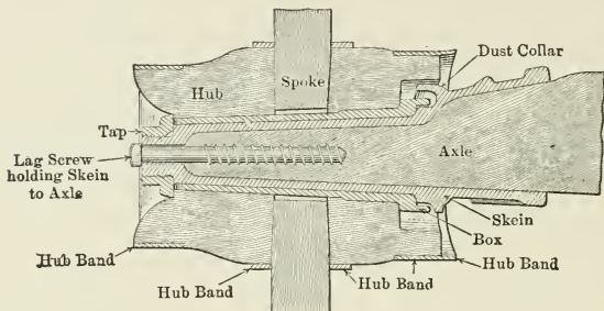
Method of attaching skein to wood axle.
