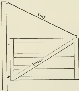
FIG. 101.—Gate guy.
