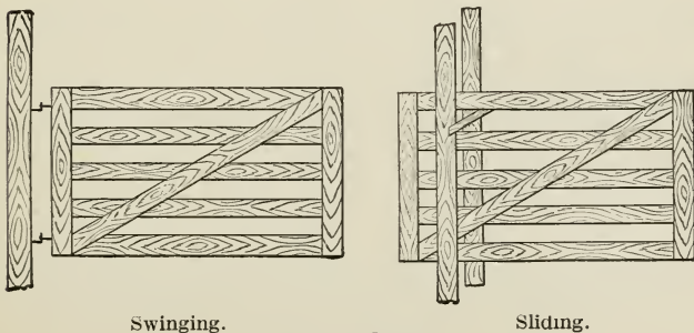
FIG. 99.—Gates.
