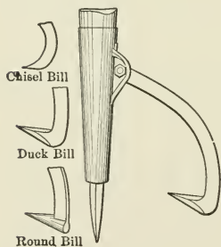
Socket peavy.
