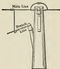
FIG. 44.—Branch-line connection. Hard-drawn copper wire.
