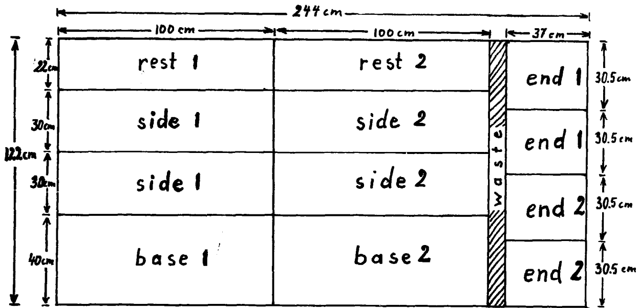
Cutting pattern for chipboard:
