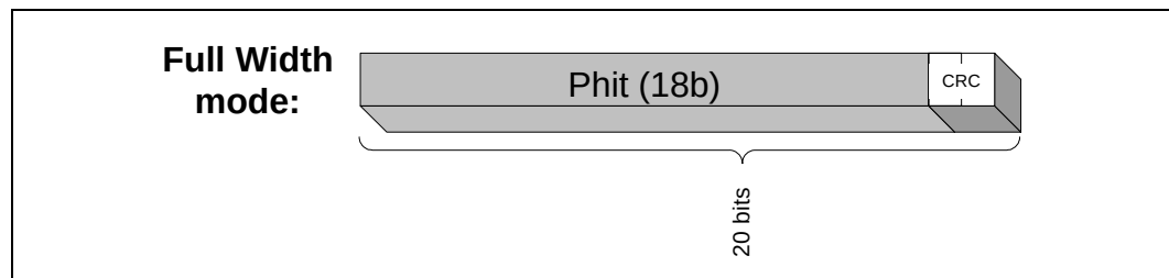
Figure 4-1. Intel® QPI Packet Visibility By The Physical Layer (Phit)
