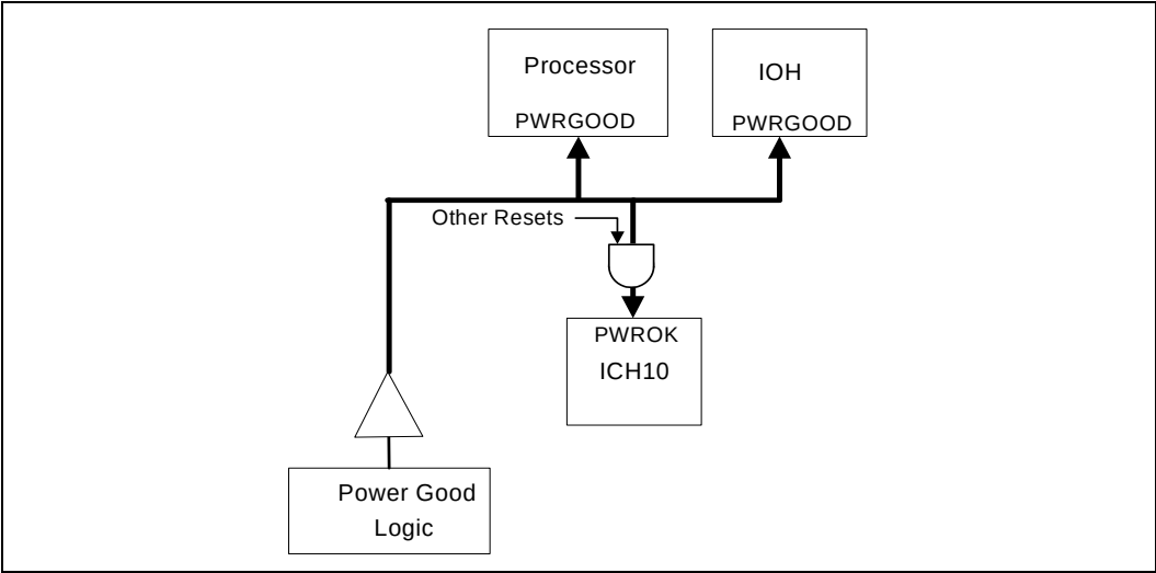
Figure 11-4. Basic System Reset Distribution
