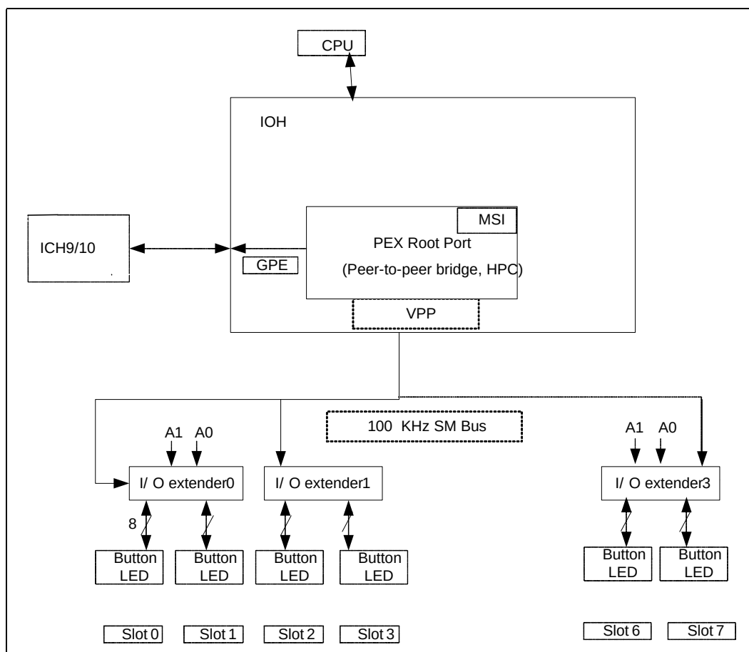
Figure 13-11. IOH PCI Express Hot-Plug Serial Interface
