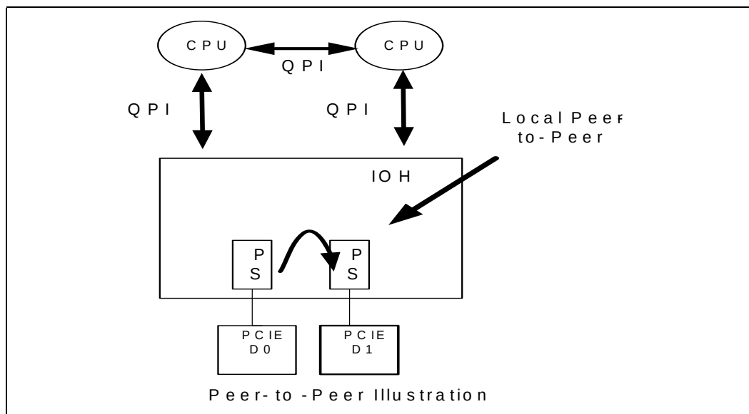
Figure 7-3. Peer-to-Peer Illustration
