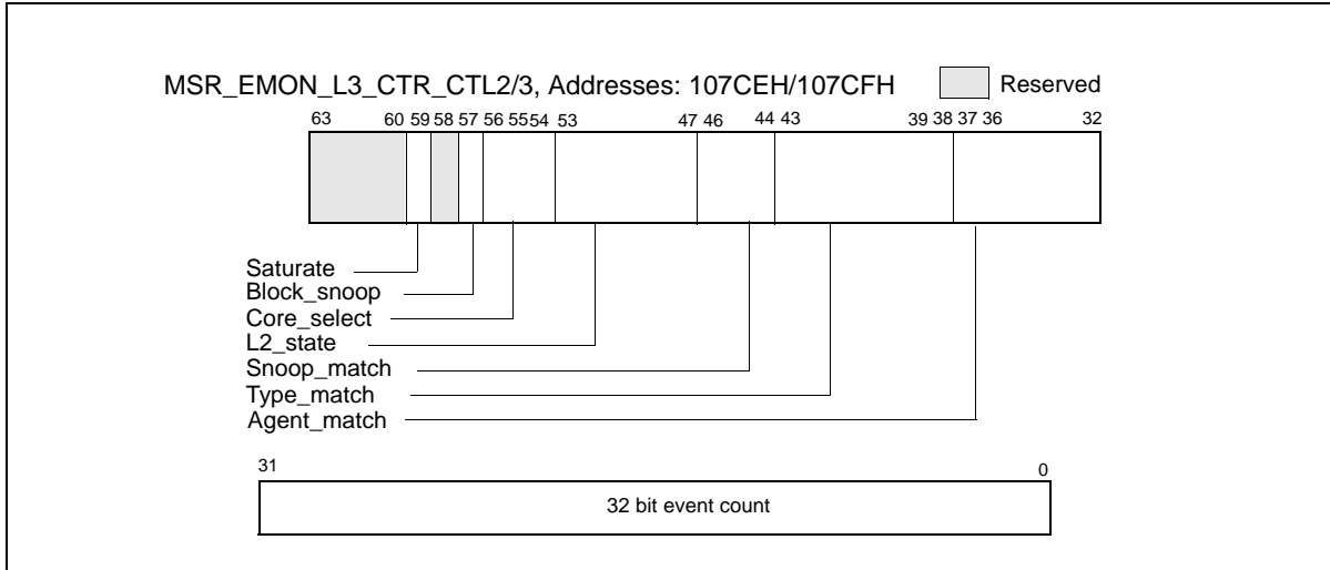
Figure 18-58. MSR_EMON_L3_CTRL2/3, Addresses: 107CEH/107CFH
