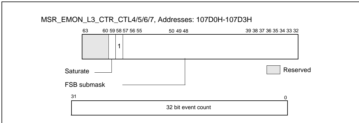
Figure 18-59. MSR_EMON_L3_CTRL4/5/6/7, Addresses: 107D0H-107D3H
