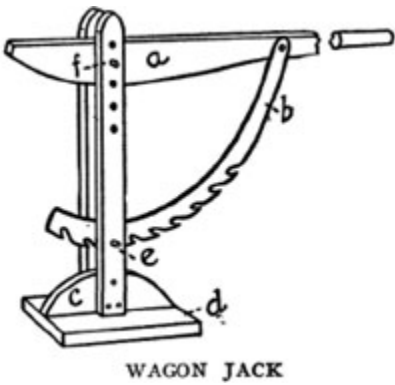
WAGON JACK
