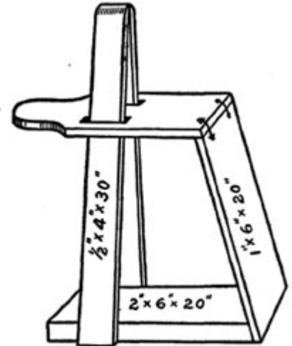
THE CLAMP
