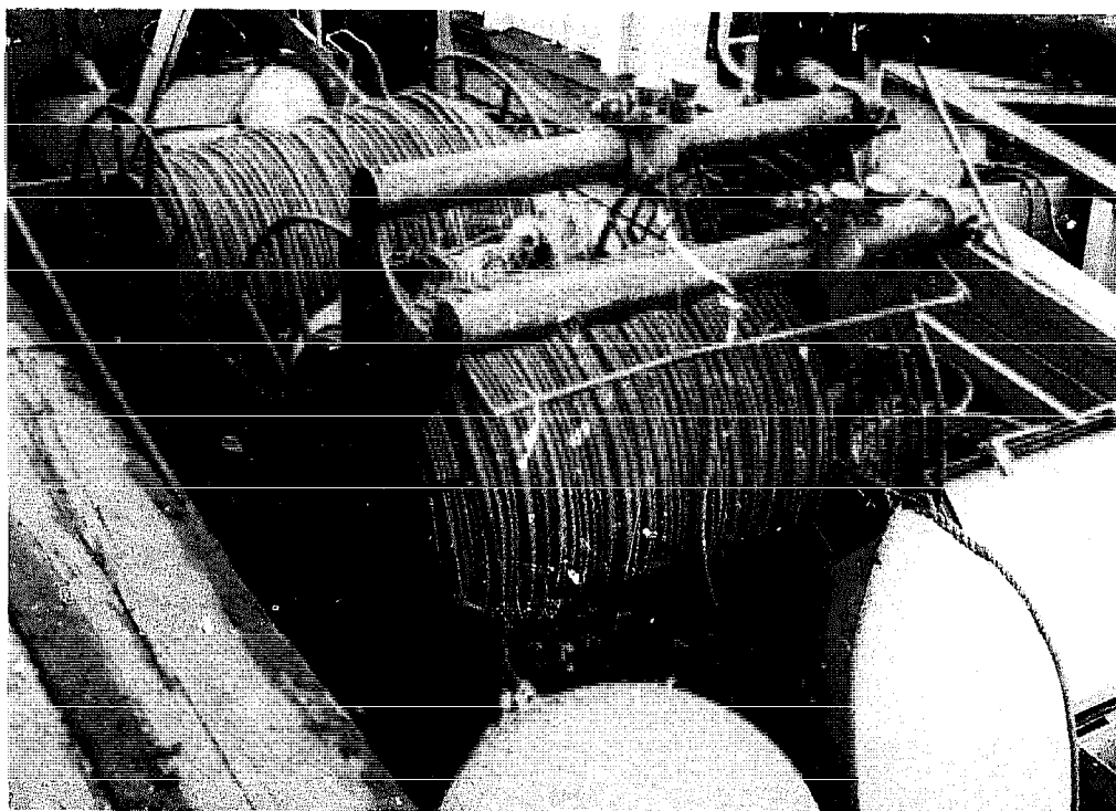
Fig 545 Modern seining with drums for the draglines Esbjerg, (1979).
