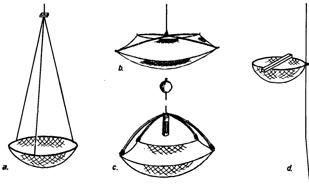
Fig 602 Various small hand liftnets: (a) crayfish ring; (b) bait net; (c) Philippine liftnet with bait box; (d) fixed crayfish net.
