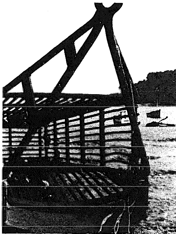
Fig 460 French dredge without teeth, which are replaced by a sharp-edged blade shearing downwards. (Photo: R Pibouhes, Brest.)
