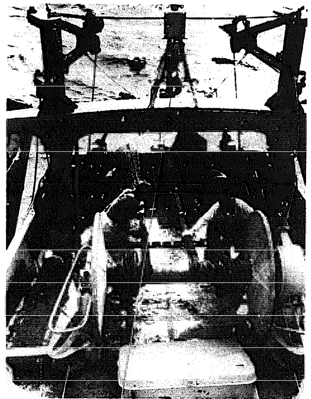
Fig 496 Hauling in the trawl with a net drum on a cutter of thirty metres in length. ( Photo: W Karger, 1970. )
