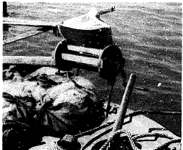
Fig 718 Simple hand-driven hauling device for trammelnets on a Greek vessel of Crete, fishing off Denia, Cyrenaica. (Photo: J Schärfe, 1961.)
