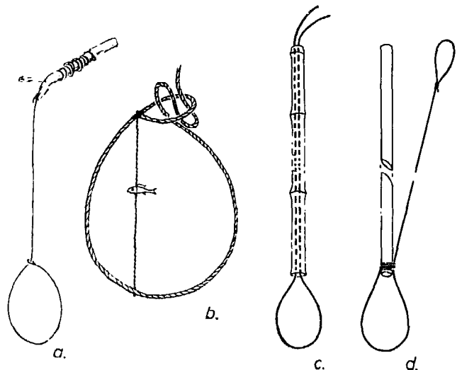
Fig 249 Fish snares: (a) Snares for sea trout used in Switzerland; (b) shark snare with bait of the Western Caroline Islands (Eilers, 1955); (c) stick snare of the Admiralty Islands (Nevermann, 1934); (d) stick snare of the Gilbert Islands (Koch, 1965).
