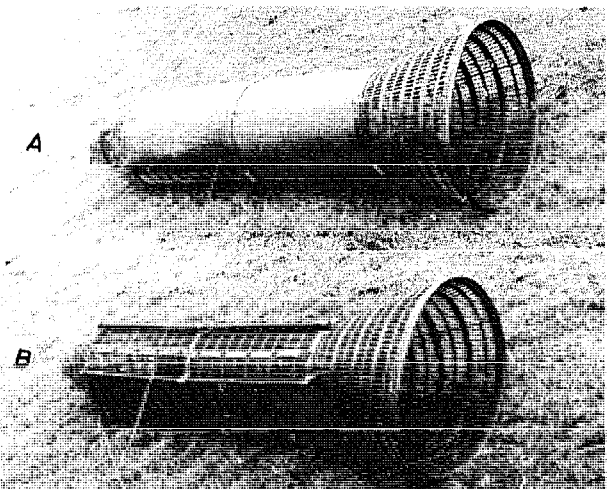
Fig 343 German eel trap made of plastic according to masterfisherman H Köthke: (a) upperside with a plate for shelter; (b) underside with two iron sticks for weighting. (Photo: G Klust.)
