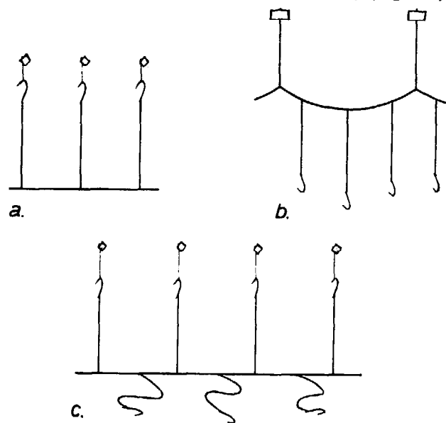
Fig 201 Different construction of sturgeon lines. The branch lines are: (a) floating; (b) hanging, or (c) alternately hanging and floating.
