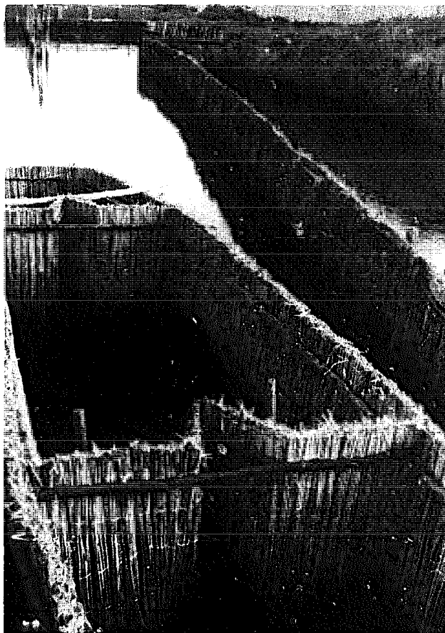
Fig 299 Catching chamber in Comacchio made of reeds (1975).
