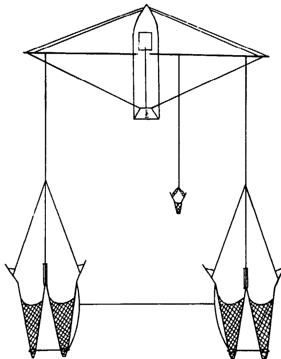
Fig 498 American double-rig shrimp trawl system. (NN, 1979).
