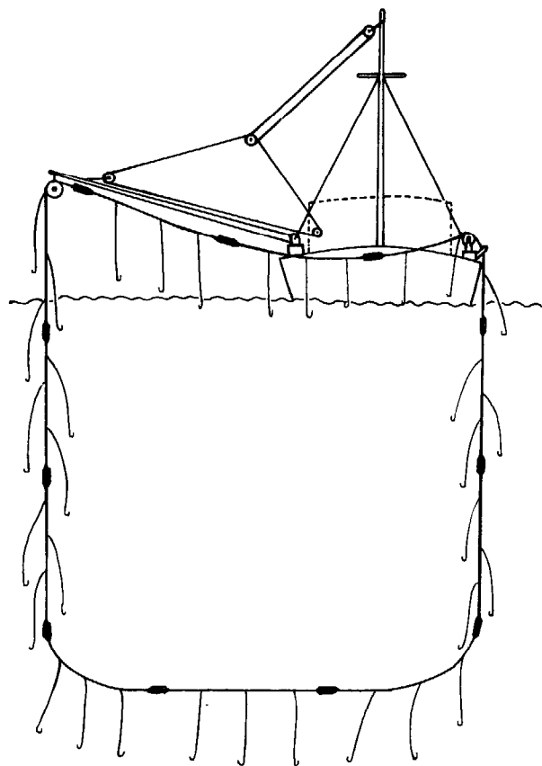
Fig 160 Modern mounting of a 'roundhauler'.
