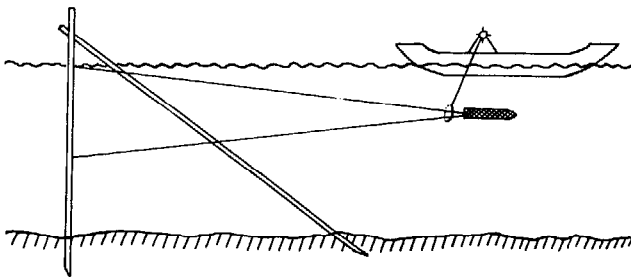
Fig 433 Stow net ending in a wooden trap behind a barrier in Kampuchea. (Fily and d'Aubentin, 1965).
