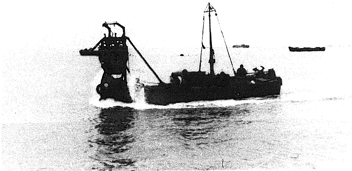
Fig 463 Italian mussel dredge in the area of Venice during transport from or to the fishing place. (1975). The dredge is mounted on the bow of the vessel.
