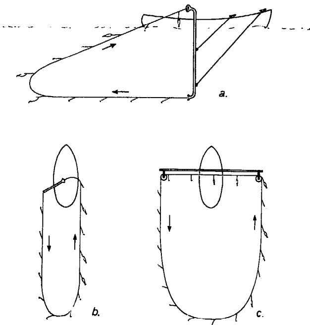
Fig 159 Mechanization of handlines: (a) Danish running line trolling; (b) Norwegian 'Atom-line-trailing'; (c) Norwegian method of handling an endless line.
