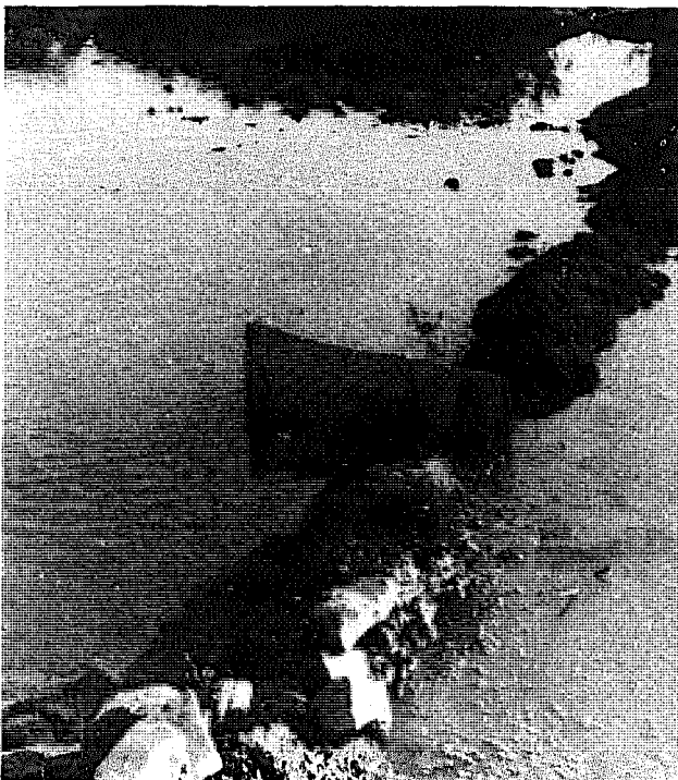
Fig 255 Temporary barrier made of mud and stones combined with a trap (Thailand, 1960).
