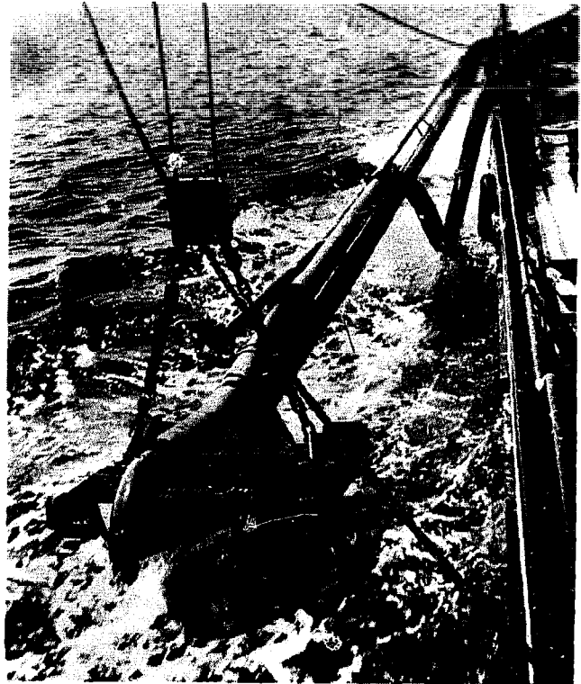
Fig 725 Dredge with high pressure hose and larger suction pipe of a British cockle dredger. (Photo: Meixner.)
