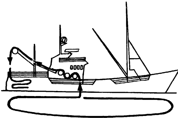
Left. Fig 581 Working diagram for hauling and transportation of a purse seine with Triplex.
