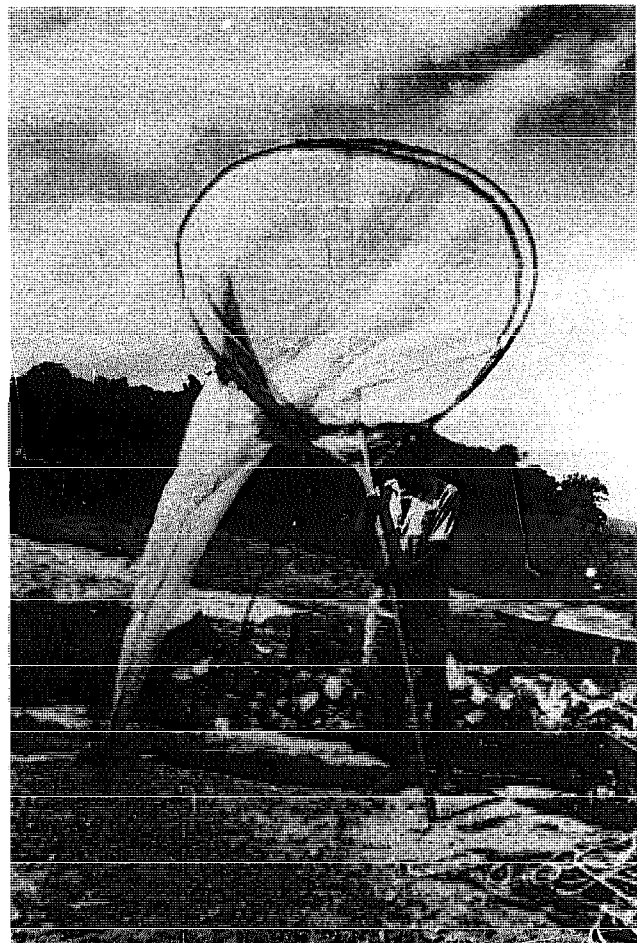
Fig 414 One of the largest hand-operated scoop nets used in night fishery with light in Lake Tanganyika. (Photo: FAO, H Kristjonsson.)
