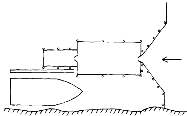
Fig 291 Barrier in Kampuchea with a small passage like a slit leading the prey into a catching chamber. (Fily and d'Aubertin, 1965).
