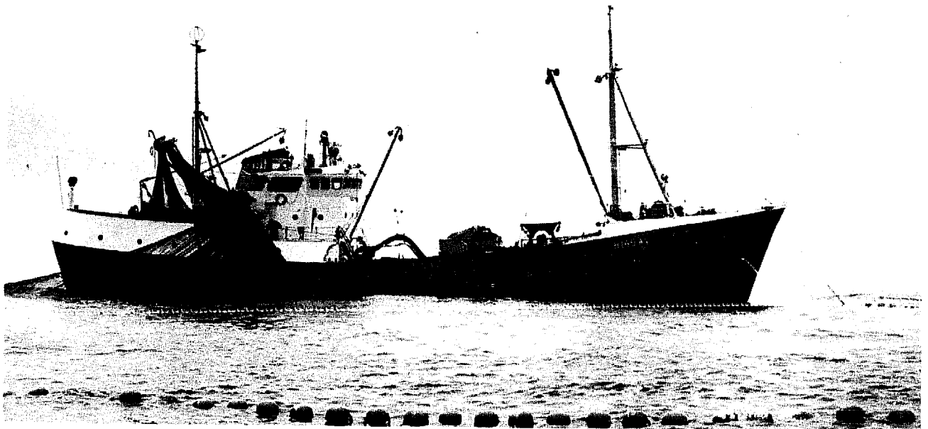
Below. Fig 582 Triplex hauling a purse seine. (Courtesy of Bjørshol Mek Werkstad, Langöyneset, Norway).
