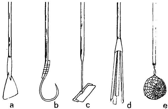
Fig 9 Long-handled tools to gather molluscs in deeper water: (a) Madagascar; (b) Japan; (c) USA; (d) Japan; (e) Thailand.
