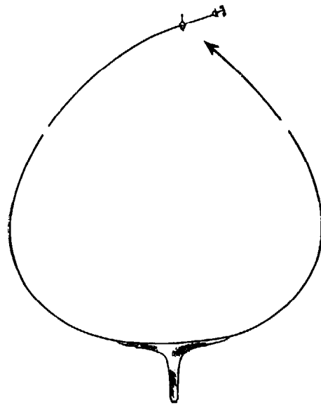
Fig 543 Danish seine net called the ‘snurrevaad’.
