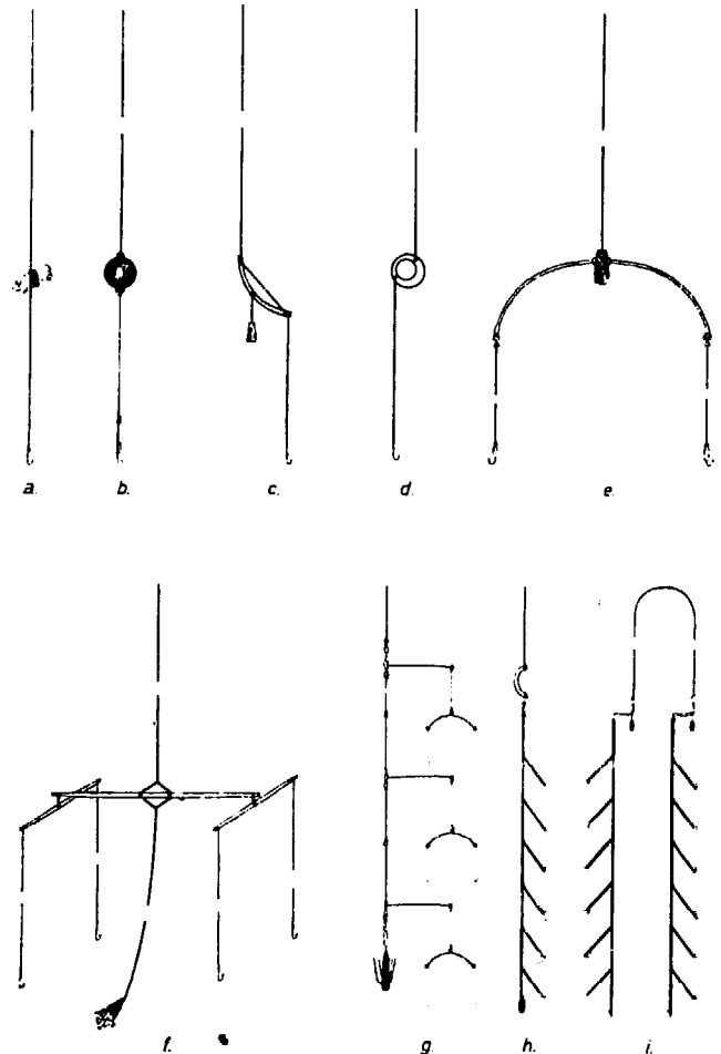
Fig 117 Handlines: (a) simple handline of Ireland; (b) handline for mackerel of Heligoland; (c) handline of Guinea ( Sahrhage, 1961 ); (d) Japanese handline with ring; (e) balance line of Faeroe Islands; (f) Icelandic handline for sharks with main and secondary balances ( Peters, 1935 ); (g) English paternoster; (h) vertical longline; (i) Chinese double handline of Formosa.
