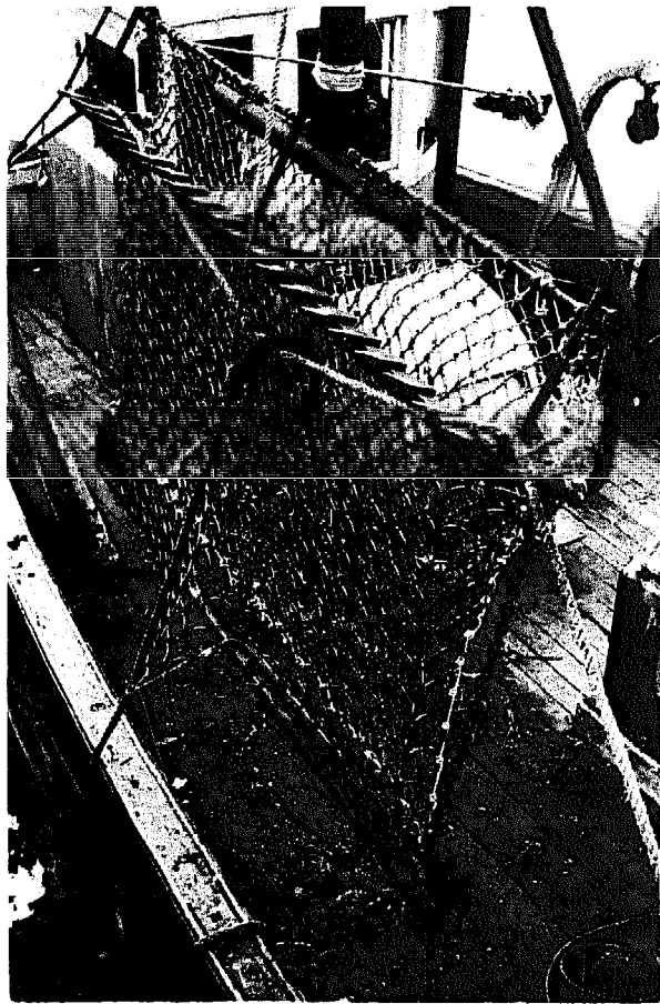
Fig 456 French dredge, Dutch type, with teeth for the collecting of venus-shells. (Photo: R Piboubes, Brest.)
