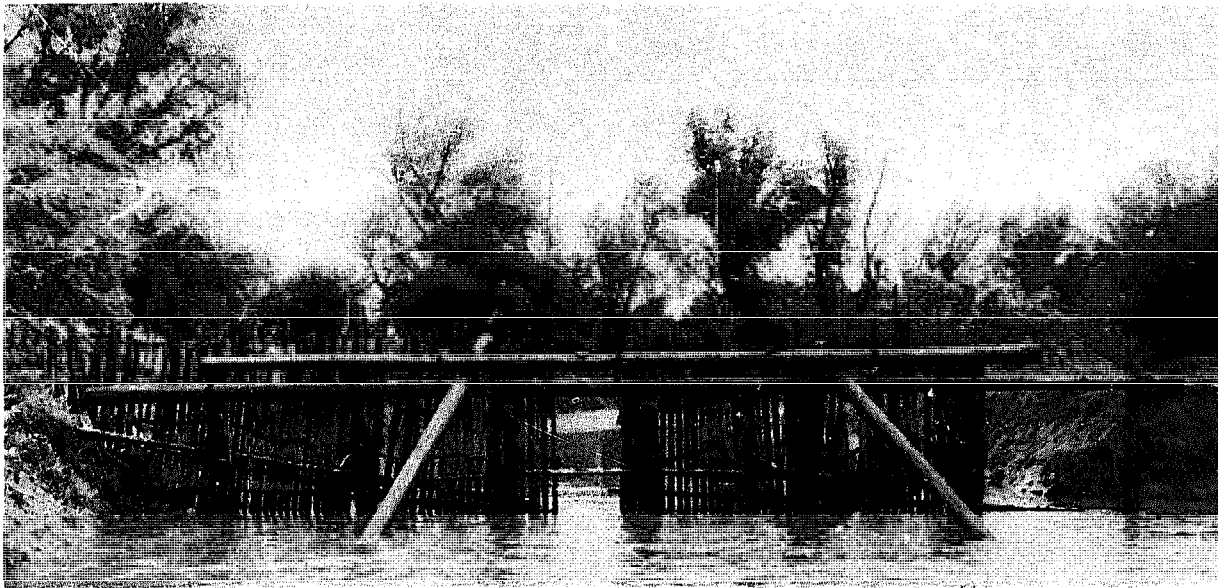
Fig 432 Barrier for stow net in the lower Danube near Braila in Rumania. In the middle of the barrier, there is a gap for the fishing gear; on the right side, an opening for passing boats (1976).
