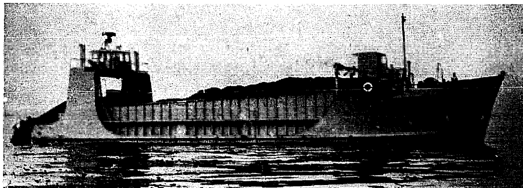
Fig 729 Modern Californian kelp harvester.
