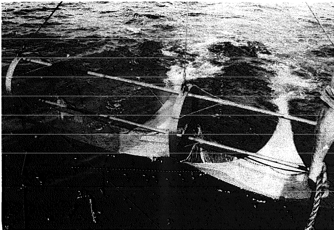
Fig 476 Agassiz trawl for making scientific catches at great depths. (Photo: H Thiel, Hamburg.)
