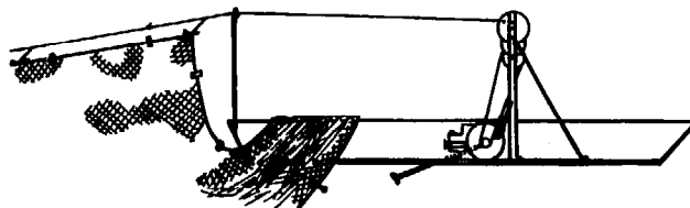
Fig 548 Motorized hauling of the wing of a seine net with an additional line as operated in Germany (1939).
