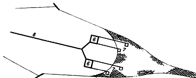
Fig 500 Sketch of electrical trawling method, according to C O Kreutzcr (Scharfe, 1965) 1. Diesel engine 2. Generator 3. Electrical impulse transmitter 4. Transformer 5. Control apparatus for impulse transmitter 6. Impulse transformer 7. Electrodes 8. Warps.
