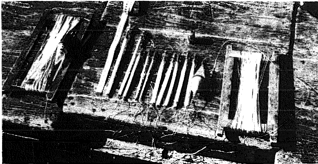
Fig 214 Chain system for different types of squid hooks beginning with an illuminated hook at the top. The longest hooks are near the bottom, Korea (1972).
