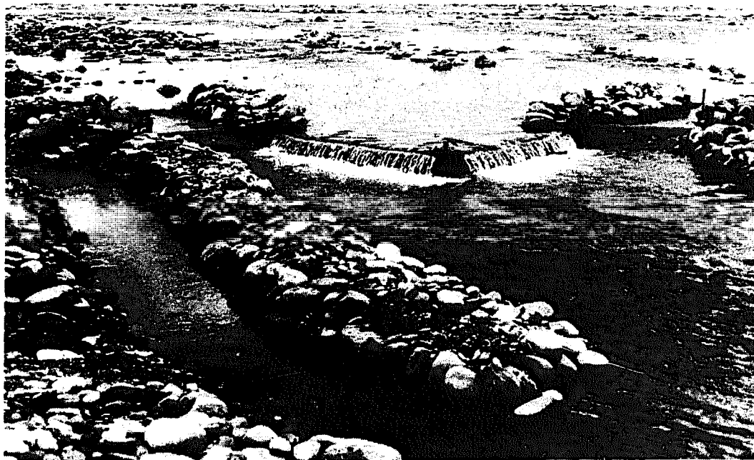
Fig 258 Barriers to catch small fish swimming against the current near Taitung in Taiwan. The fish are not caught in the middle cascades with strong currents but in the slower water on both sides.
