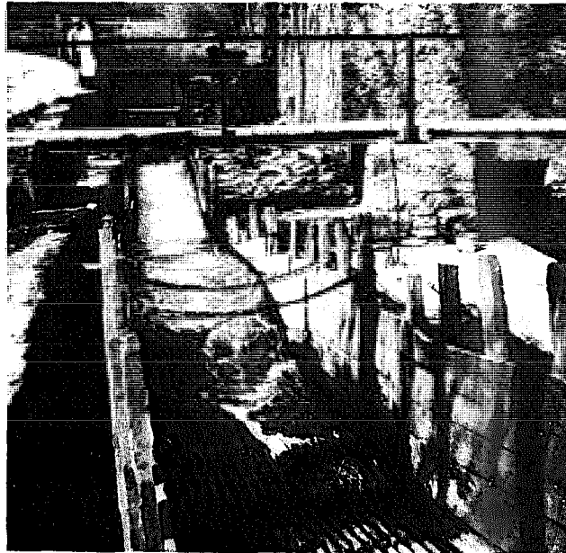
Fig 266 Gratings for catching eels in the outlet of a mill-pond in the Eifel/Germany. (Photo: G Jens.)
