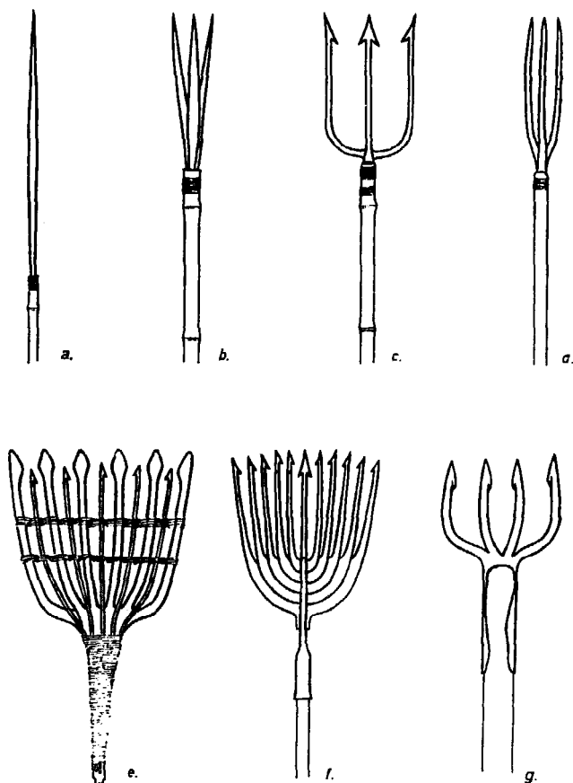
Fig 39 In every corner of the world fishing spears were evolved: (a) simple fish-stick of Guinea; (b) fish spear with three points arranged as a bundle; (c) trident spear with barbs; (d) Arabian spear of Syria, without barbs; (e) fish spear of Northern Germany; (f) Italian spear for cuttlefish; (g) spear for sponge fishing off the coast of Libya.
