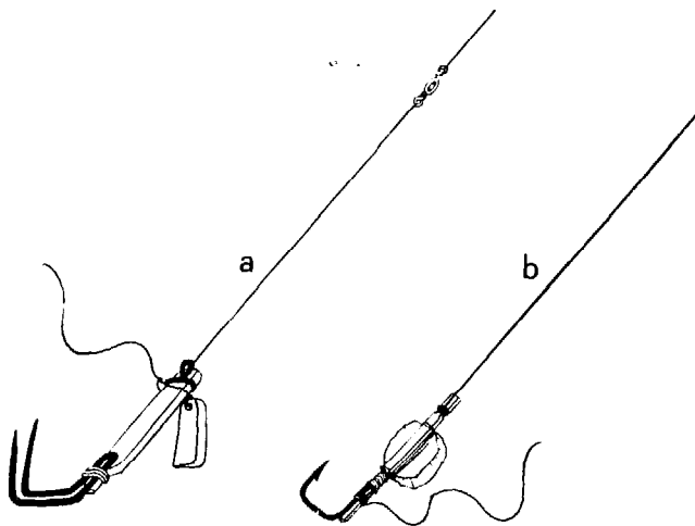
Fig 218 Korean ripping handlines for catching octopi: (a) for pilking from an anchored vessel; (b) ripping troll line (1979).
