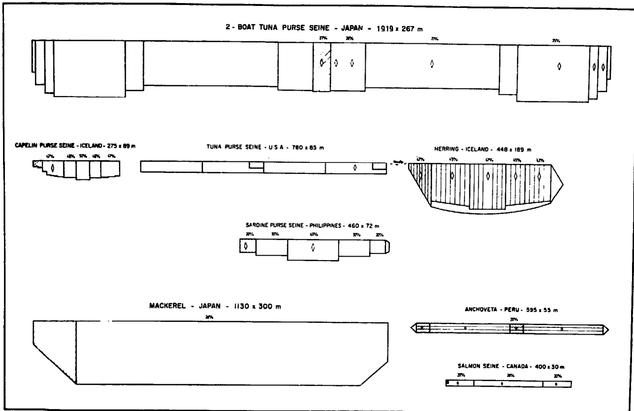
Fig 562 Comparison of the size of different types of one-boat and two-boat purse seines. (H Kristjonsson, 1971).
