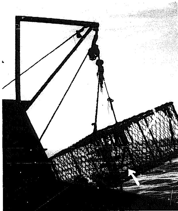
Fig 337 Hauling a rocklobster pot near Akaroa, New Zealand. To prevent the prey escaping long spines are welded around the entrance of the trap. The arrow shows the escape vent on the back of the trap (1981).
