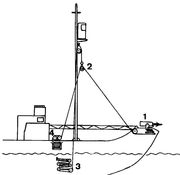
Fig 66 Leading a harpoon line from the gun (1) over a block (2) hanging on the mast and connected to a tension absorber (3). The line is coiled with the whale winch (4) and stored in the hold of the vessel.
