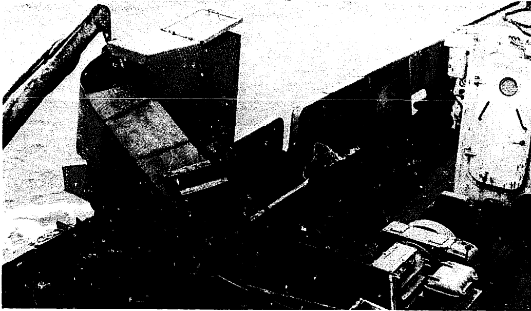
Fig 721 Pump and separator for 'kilka' fishing on the Russian vessel Lenkoram , fishing in the Caspian Sea.
