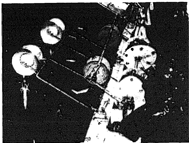
Fig 220 Japanese automatic squid angling machine in operation.
