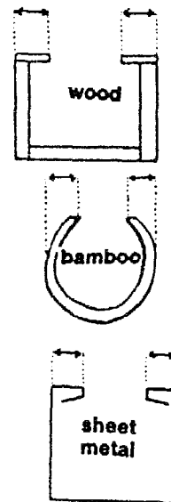
Fig. 16,17,18. Lip overhang
