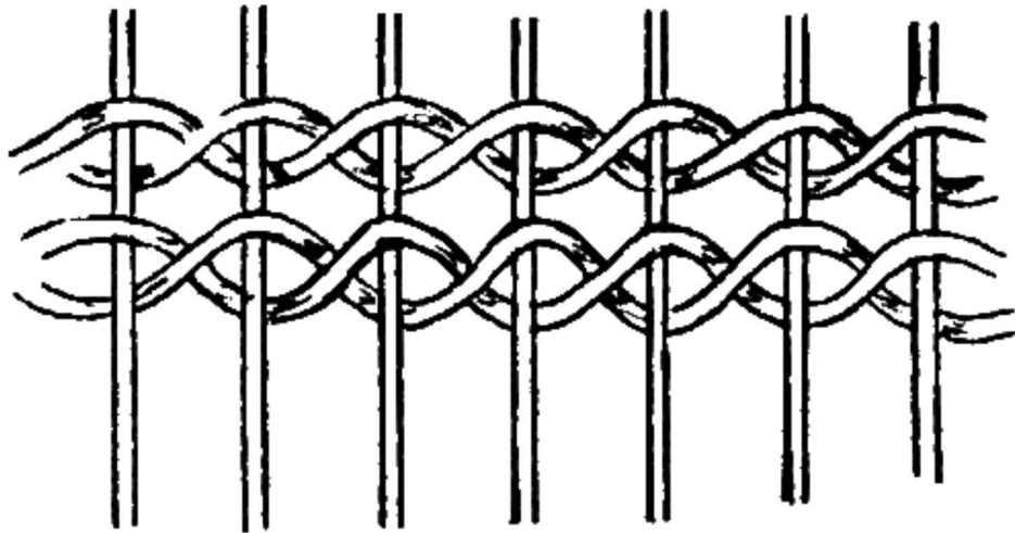
DIAGRAM NO. 3.—PAIRING
