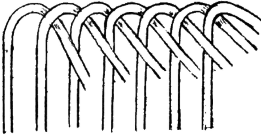
DIAGRAM NO. 16.—CLOSED BORDER NO. 1 (PART 1)
