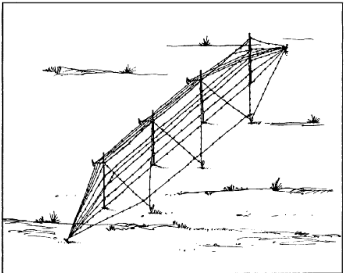
Figure 2-10. Double-apron barbwire fence.
