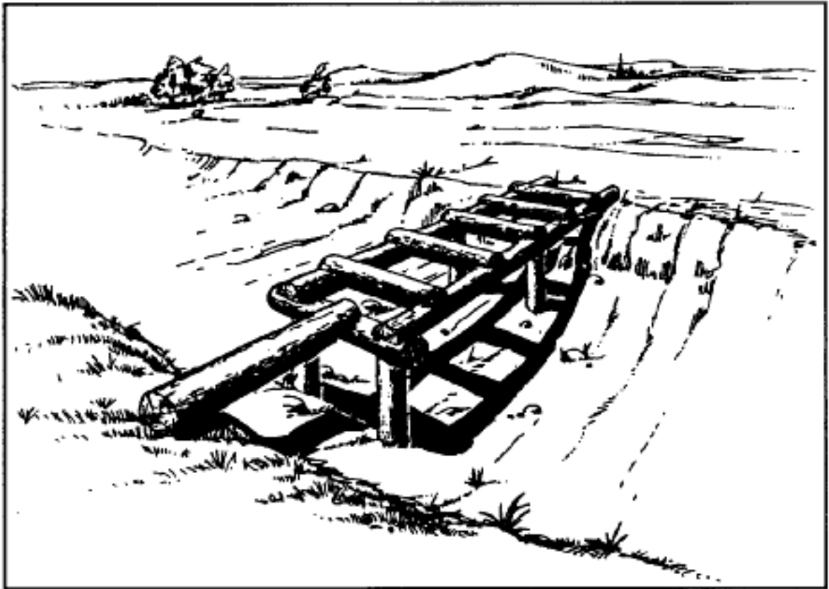
Figure 2-7. Log balance and horizontal ladder.
