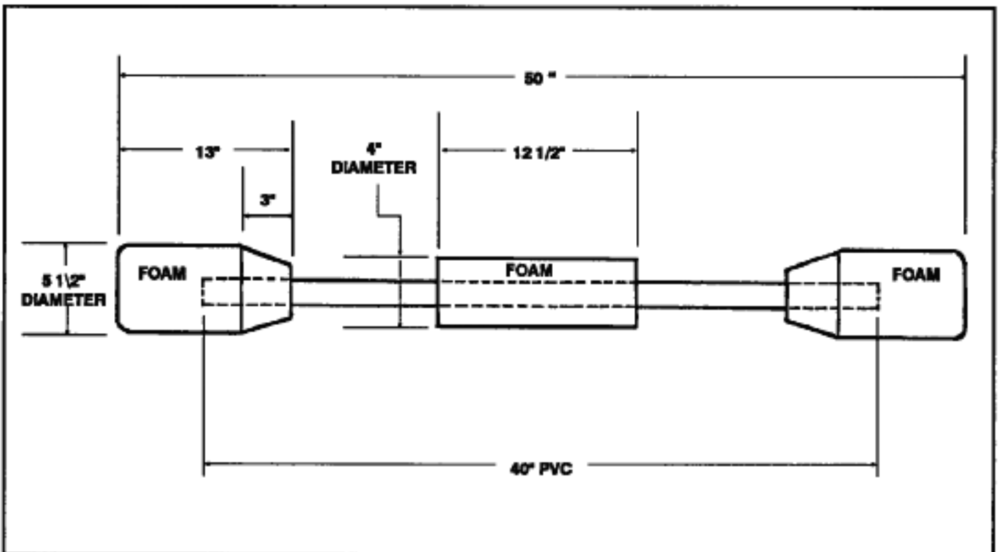
Figure A-6. Materials in pugil stick construction.
