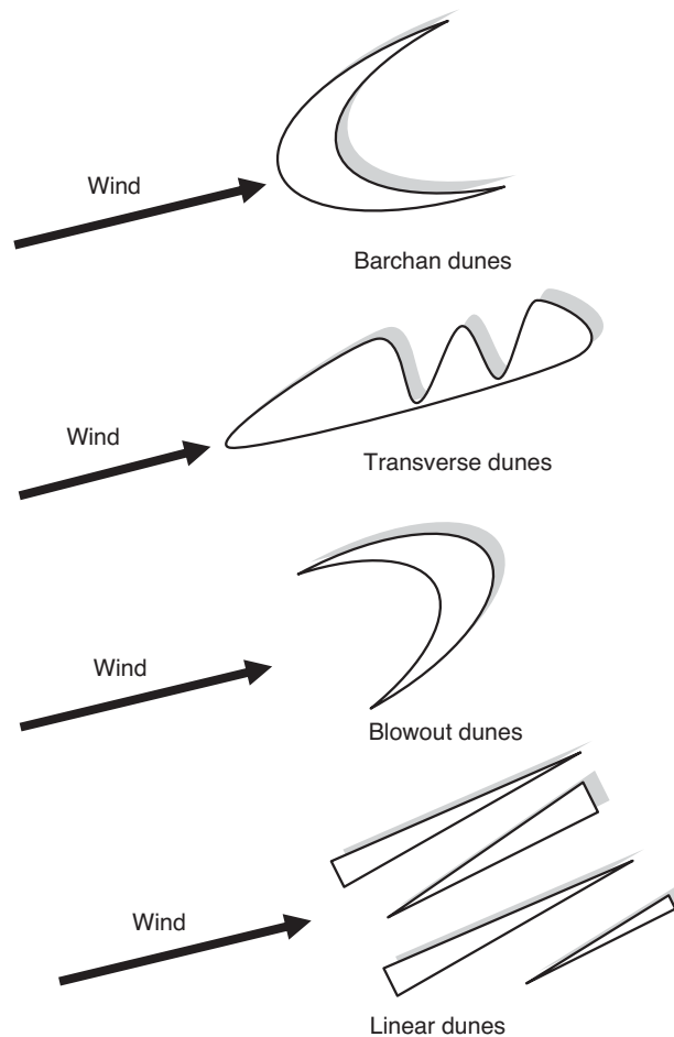
Fig. 10-4 There are four main types of sand dune formations.
