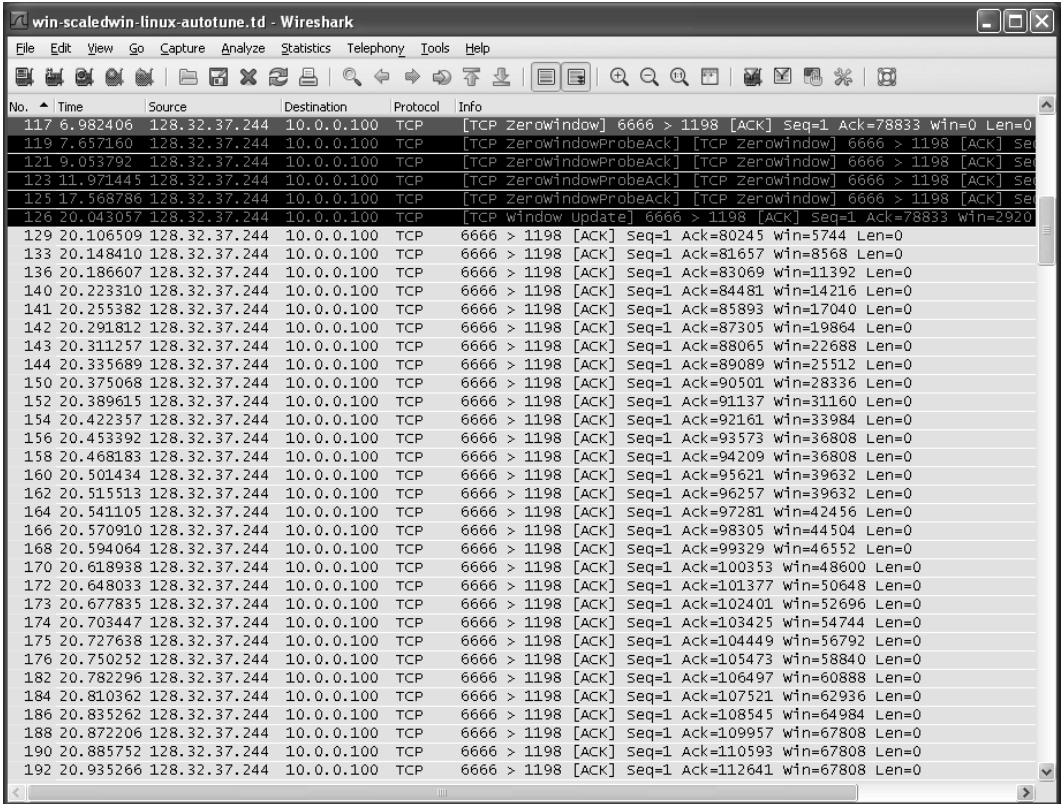
Figure 15-16 With the application pausing before reading, auto-tuning is compromised because the receive buffer becomes full. As the application begins reading, the advertised window increases, exceeding its previous value.
