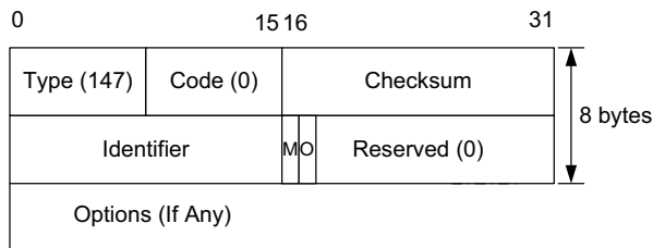
Figure 8-22 The MIPv6 Mobile Prefix Advertisement message. The Identifier field matches the corresponding field in the solicitation. The M (Managed) flag indicates that the address is provided by a stateful configuration mechanism. The O (Other) flag indicates that other information beyond the address is supplied by stateful mechanisms.
