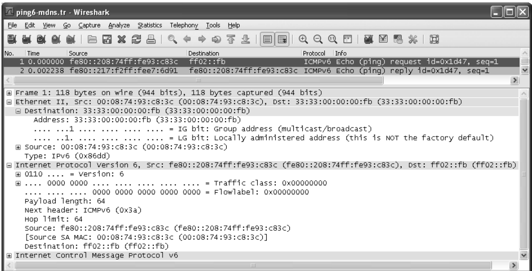
Figure 9-4 An ICMPv6 Echo Request message is sent from a link-local unicast address associated with the eth0 network interface to the multicast address ff02::fb. The reply includes the sender's IPv6 link-local IPv6 address.
