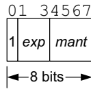
Figure 8-27 The MLDv2 Querier's Query Interval Code encodes the interval between MLDv2 queries. The (unencoded) version of this value is called the Querier's Query Interval and is measured in seconds. The QQI is computed as follows: QQI = QQIC (if QQIC < 128 ) and QQI = ((mant \mid 0x10) \ll (exp + 3)) otherwise.
