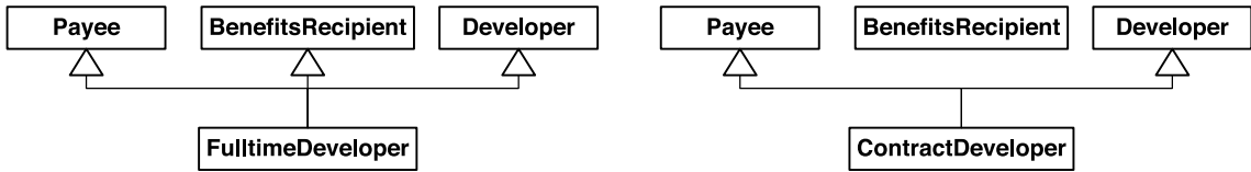
Figure 4-3. Example of bad inheritance
