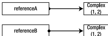
Figure 13-2. References to ComplexNumber
