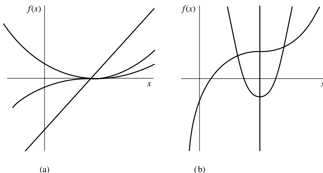
Figure 9.5.1. (a) Linear, quadratic, and cubic behavior at the roots of polynomials. Only under high magnification (b) does it become apparent that the cubic has one, not three, roots, and that the quadratic has two roots rather than none.
