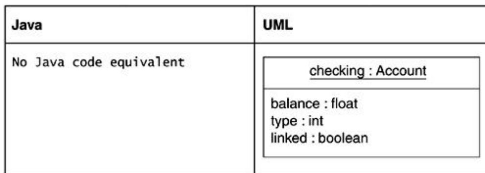
Figure 4-5. An object
