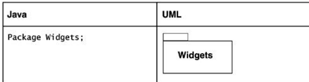
Figure 4-8. A package
