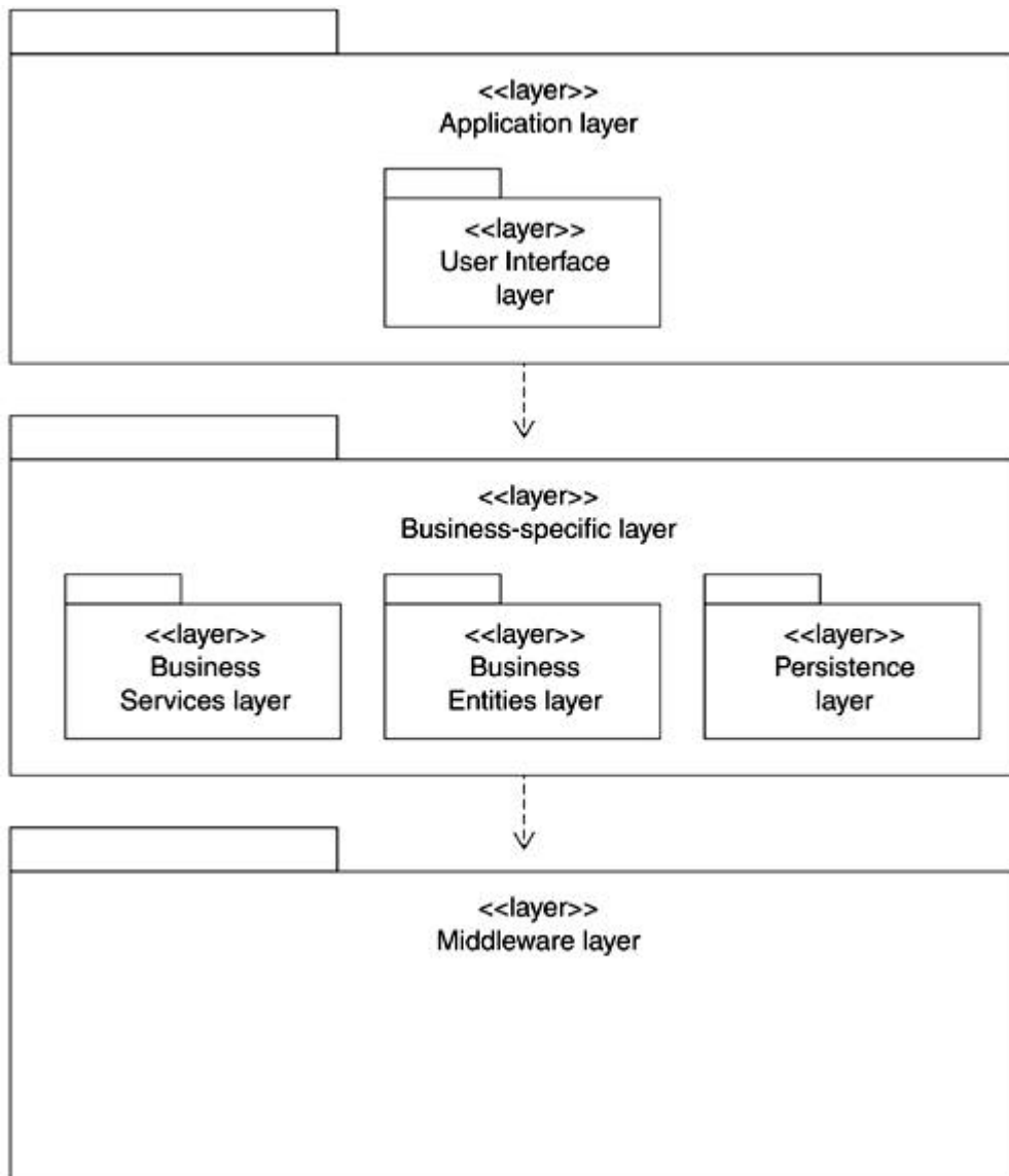
Figure 13-23. Layering
