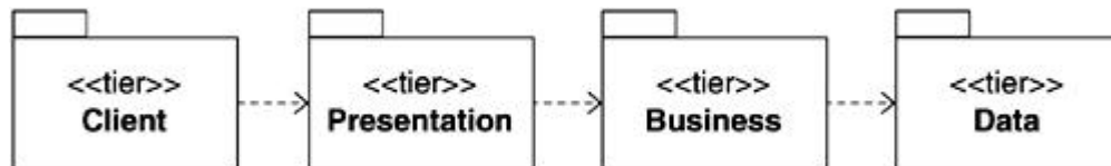
Figure 6-8. J2EE tiers
