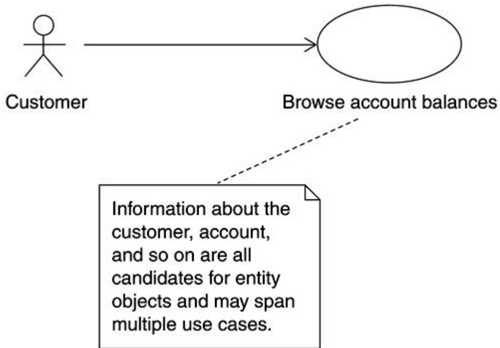
Figure 8-4. Entity objects and use cases
