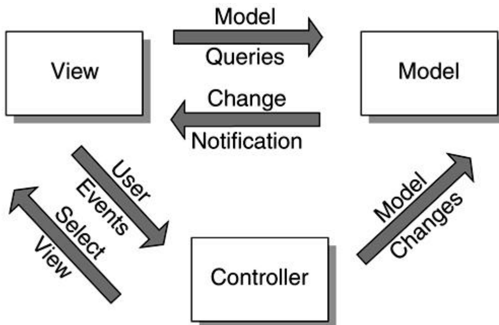
Figure 2-4. Model-View-Controller architecture
