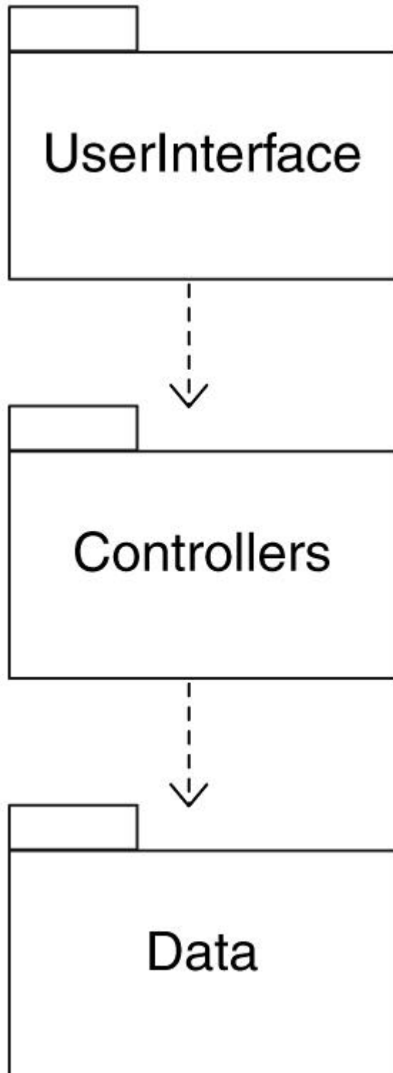
Figure 8-13. Package dependency
