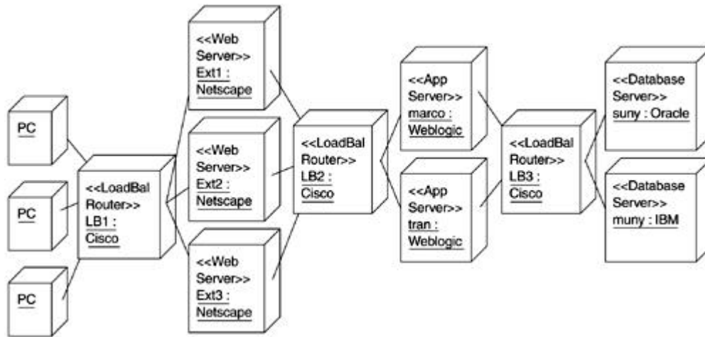
Figure 15-8. Redundancy modeling via deployment diagram
