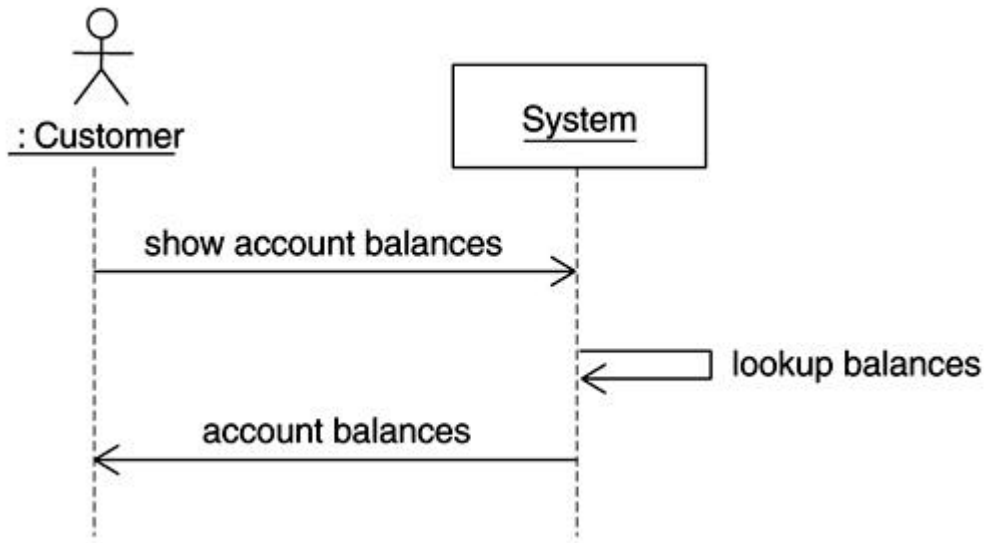
Figure 16-3. Browse account balances main flow of events
