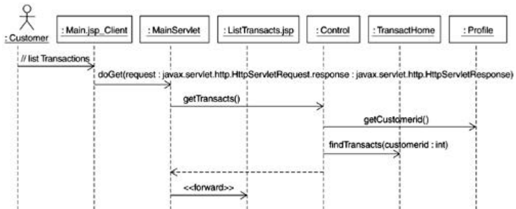
Figure 16-6. List transactions main scenario sequence diagram
