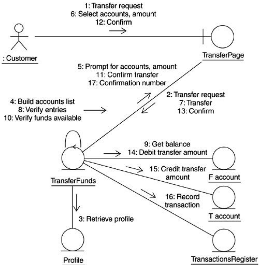
Figure 8-8. Transfer funds collaboration diagram
