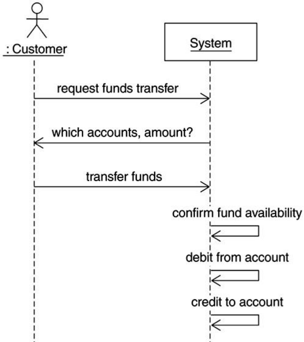
Figure 16-4. Transfer funds main flow of events
