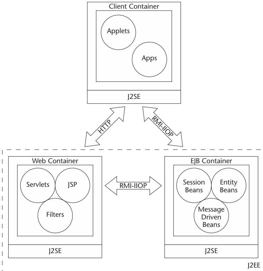
Figure 37.5 Java containers.
