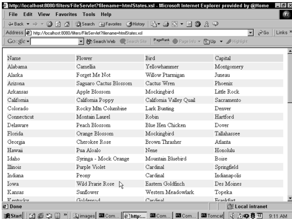
Figure 28.2 XSLT output.
