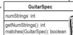
GuitarSpec.java
