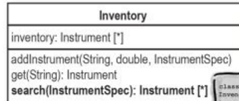
Inventory.java
