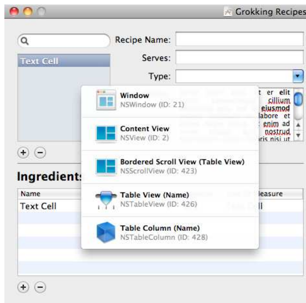
Figure 2.8: List view tree
