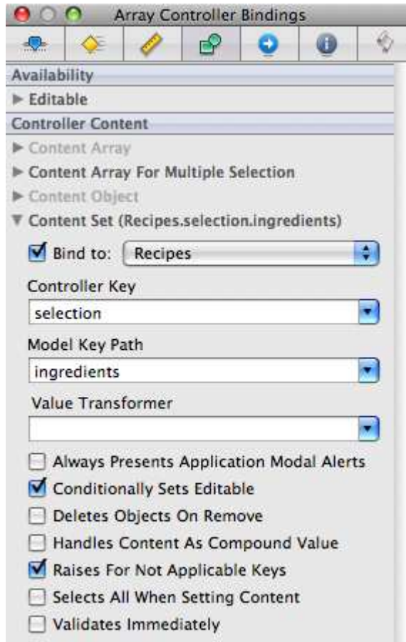
Figure 2.6: NSArrayController content set properties
