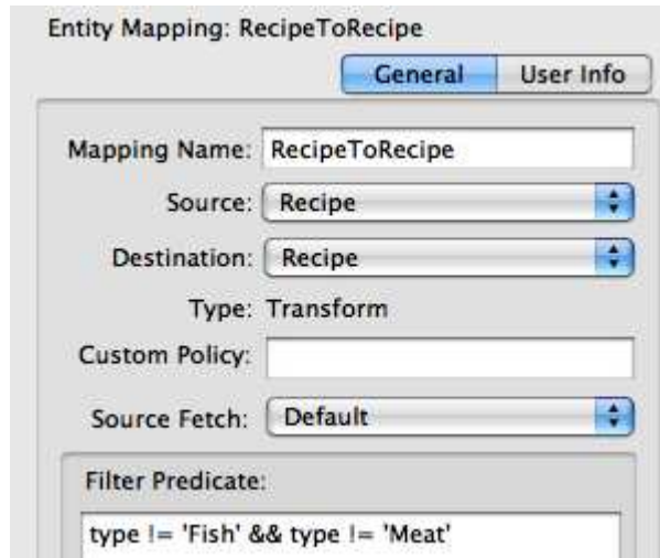
Figure 5.6: Exclusion filter predicate
