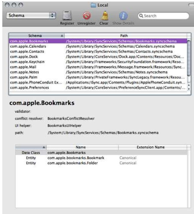
Figure 8.4: Syncrospector Schema pane
