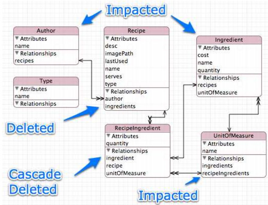
Figure 6.4: Impacts of deleting a recipe
