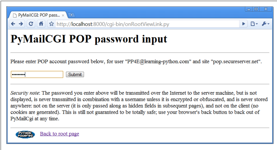
Figure 16-7. PyMailCGI view password login page
