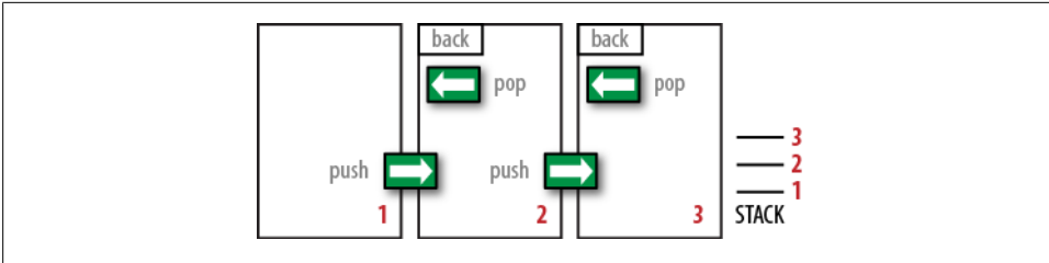
Figure 16-5. Breadcrumb navigation flow and view stack
