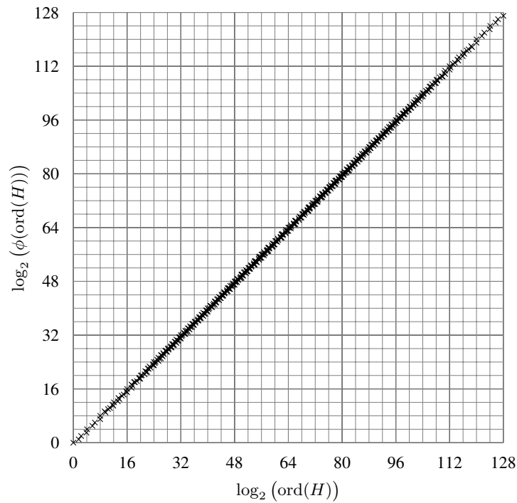
Fig. 1. The orders of 512 the multiplicative groups in GF(2^{128}) are marked with small crosses. The Euler totient function \phi(\text{ord}(H)) indicates the number of elements that belong the given subgroup but not its subgroups.
