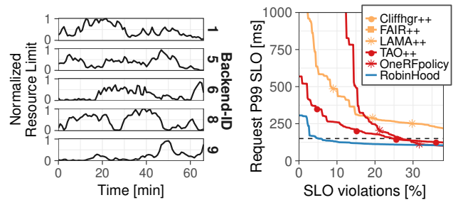
(a) Randomized Resource Limits. (b) SLO violations.
